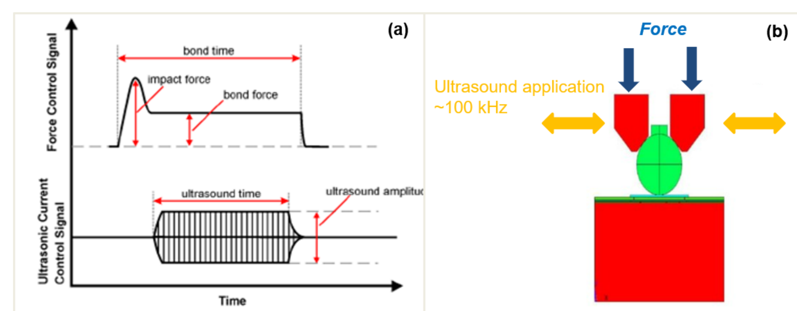
Figure 3: Detailed figuration of wire/device pad interaction in wire bonding process. In (a), the dynamic force and ultrasound profiles are depicted, while in (b) the force application on ball is sketched.
