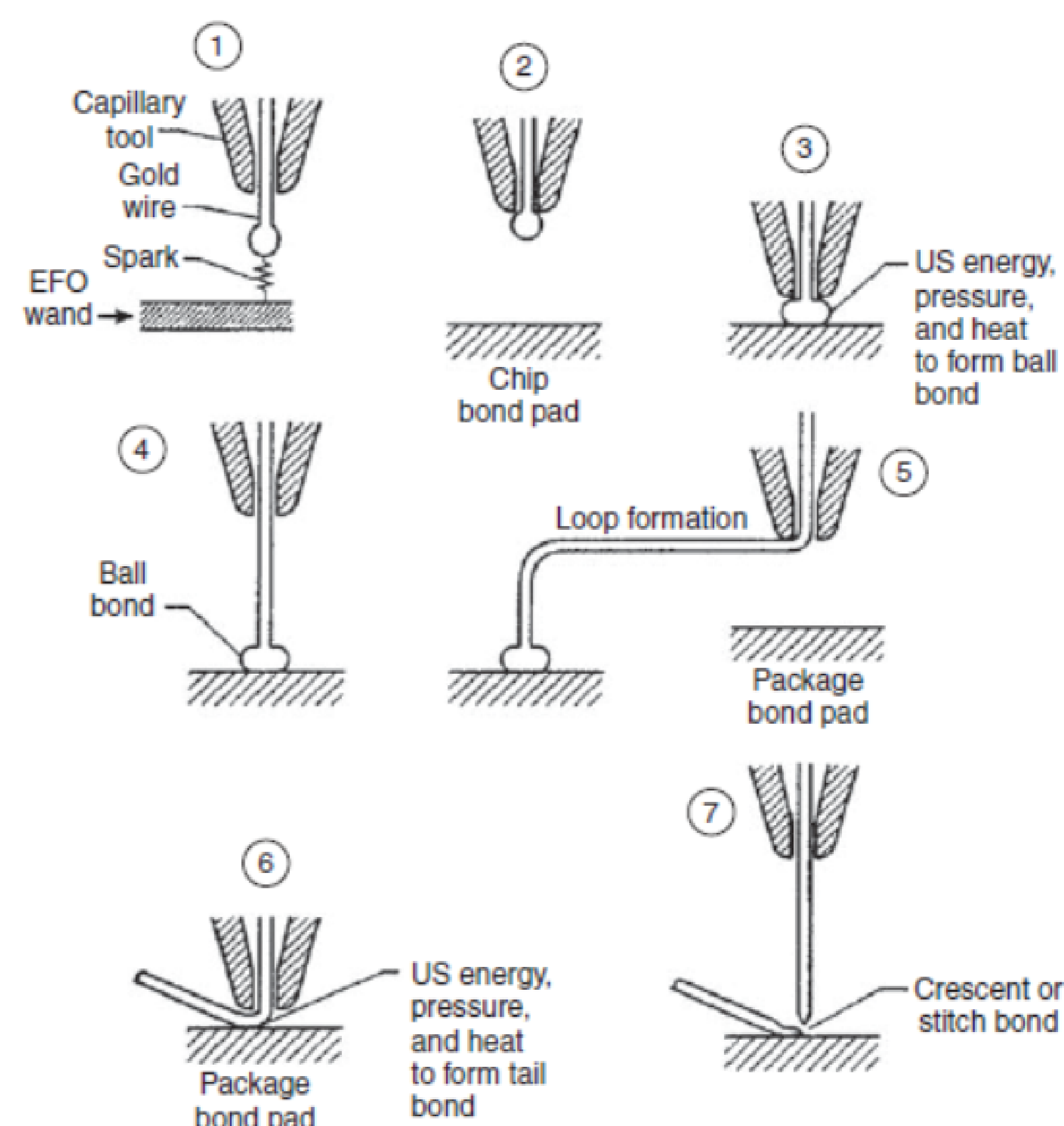
Figure 2: Typical process flow for wire bonding (from Chauhan, P.S., "Copper Wire Bonding")
